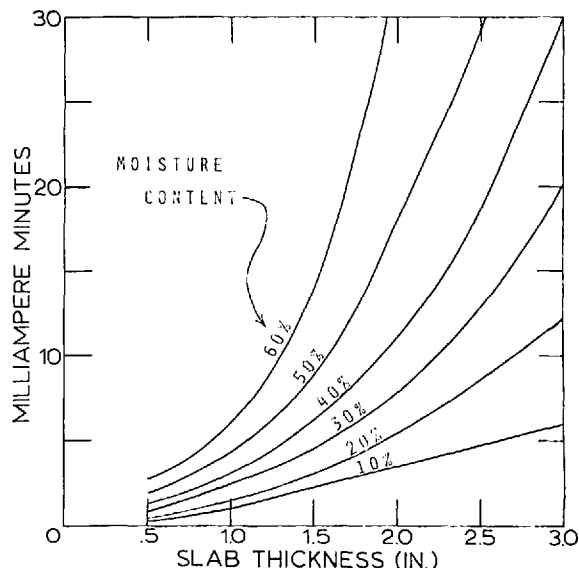
FIG. 1.—X-ray exposure curves for wood-and-bark slabs of different thickness and moisture content when the X-ray unit is operating at 25 kv, 5 ma, using a 20-in. target-to-film distance.
