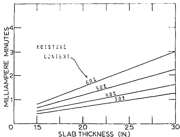
FIG. 2.—X-ray exposure curves for wood-and-bark slabs of different thickness and moisture content when the X-ray unit is operating (without filter) at 45 kv, 5 ma, using a 20-in. target-to-film distance.
